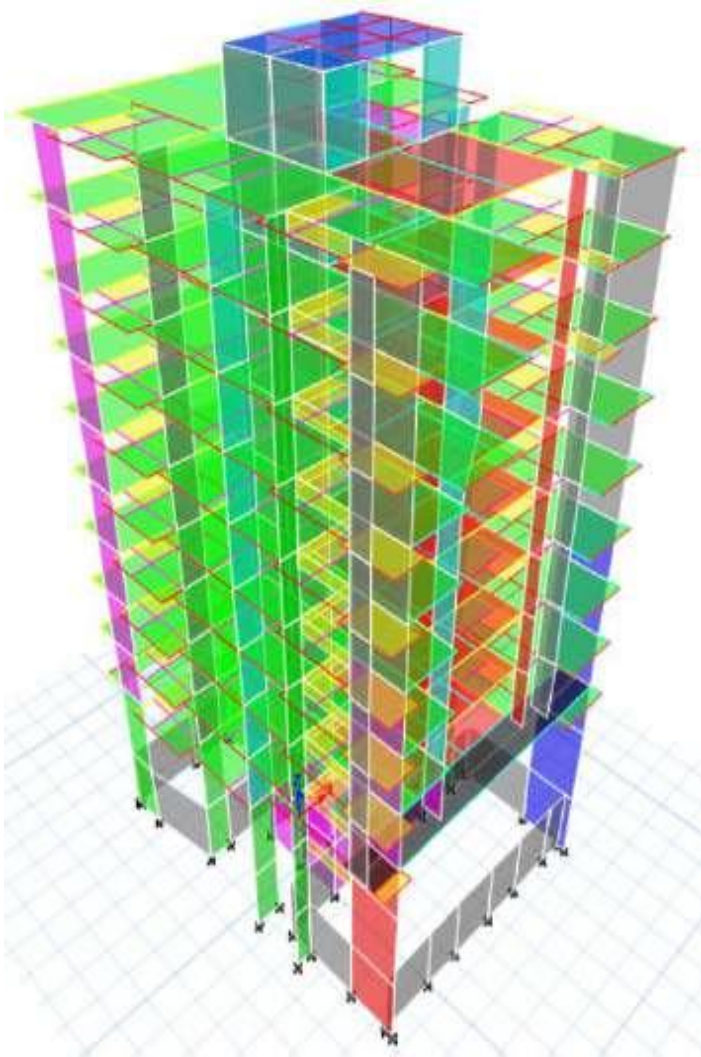
ONKAR RESIDENTIAL PROJECT MUMBAI [G+9]
